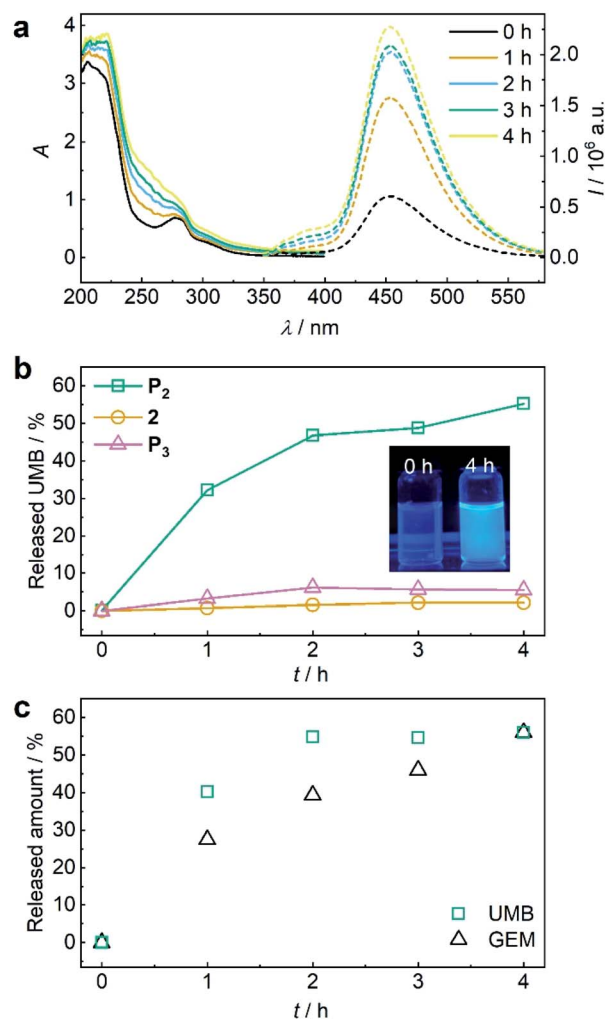
Fig. 5 US-induced release of UMB and GEM from \beta -carbonate disulfide polymer P 2 ( 3 \text{ mg mL}^{-1} ) and control 2 ( 25 \mu\text{M} ) in MeCN : H 2 O = 2 : 3 (v/v). (a) UV-vis and fluorescence ( \lambda_{exc} = 325 \text{ nm} ) spectra of P 2 during sonication. (b) Released UMB from P 2 and controls 2 and P 3 during sonication calculated from fluorescence peak intensity of UMB at \lambda_{em} = 450 \text{ nm} . Inset: photograph of the solutions under UV-light ( \lambda_{exc} = 365 \text{ nm} ). (c) Released amount of UMB and GEM over time visualized by PDA detector signal intensities from UPLC elugrams (Fig. S46 † ).
