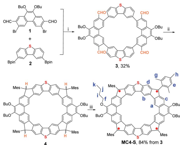
Scheme 1 Synthetic route of MC4-S : (i) \text{Pd}_2(\text{dba})_3 , [(t\text{-Bu})_3\text{PH}]\text{BF}_4 , \text{NaHCO}_3 , THF/ \text{H}_2\text{O} , 80 °C; (ii) (1) \text{MesMgBr} , THF; (2) \text{BF}_3 \cdot \text{OEt}_2 , DCM; (iii) DDQ, toluene.
