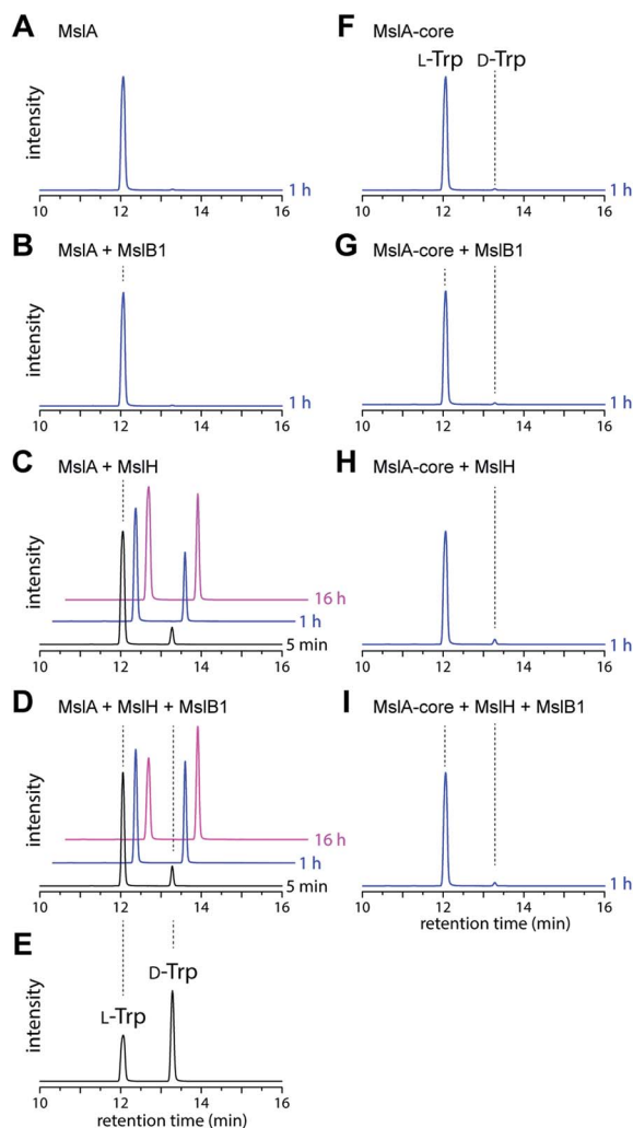
Fig. 3 LC-MS analysis (ESI negative ion mode, y-axis is signal intensity monitored at m/z 497 and the same scale applies for all chromatograms) of L-FDLA-Trp derived from in vitro reactions. The reaction time is shown next to each trace. (A) MslA only, (B) MslA + MslB1, (C) MslA + MslH, (D) MslA + MslH + MslB1, (E) L- and D-Trp standards, (F) MslA-core only, (G) MslA-core + MslB1, (H) MslA-core + MslH, and (I) MslA-core + MslH + MslB1.
