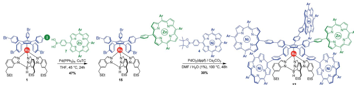
Scheme 5 Synthesis of the chemically-tagged cogwheel 12 , incorporating one distinct zinc(II) porphyrin (in green), via sequential chemoselective Suzuki–Miyaura cross-coupling reactions. Ar = 3,5-di- tert -butylphenyl.
