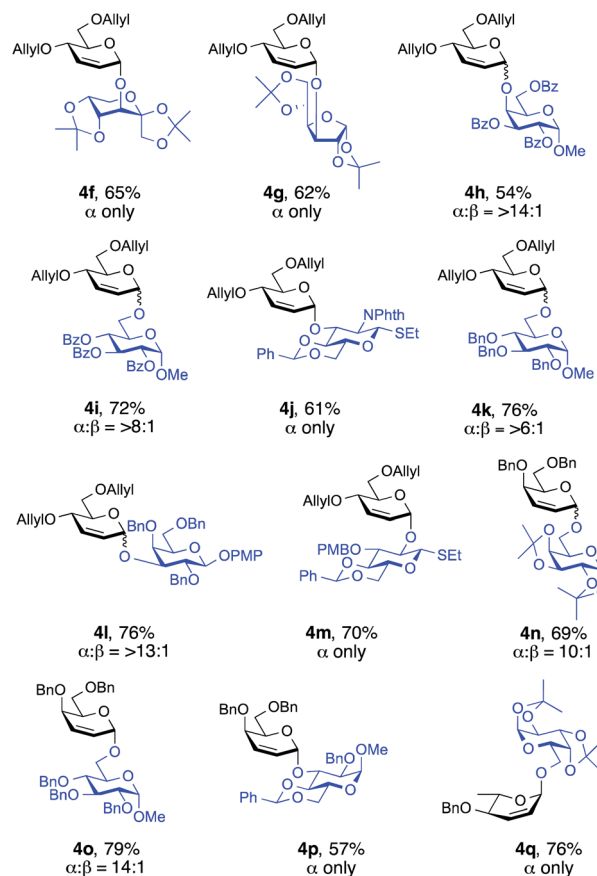
Fig. 2 α-Selective Ferrier type O -glycosylation of 1n , 1u and 1v with a variety of glycosyl acceptors. Reactions were carried out under a N 2 atmosphere using 1.5 equiv. glycosyl donor ( 1 ), 1.0 equiv. of acceptor ( 2 ), 3.5 mol% [Ir(COD)Cl] 2 , 14.0 mol% AgOTf, and 1.0 equiv. of Ag 2 CO 3 in dry CH 2 Cl 2 for 48–72 h at rt. Stereoselectivity was determined by crude 1 H NMR. Isolated yields.
