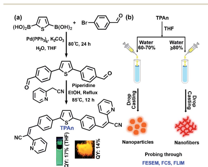
Fig. 1 (a) Synthetic route for TPAn involving Suzuki coupling between thiophene-2,5-diylboronic acid and 4-bromobenzaldehyde, followed by Knoevenagel condensation between C–C coupled product, 4,4'-(thiophene-2,5-diyl)dibenzaldehyde and 2-pyridylacetonitrile. The digital photographs demonstrating strong emission of TPAn in solution and powder under the illumination at 365 nm; respective fluorescence quantum yields (QY) are mentioned. (b) Schematic illustration depicting the formation of TPAn nanoparticles and nanofibers with varying the composition of the THF–water mixture probed through a combined microscopic and spectroscopic approach.
