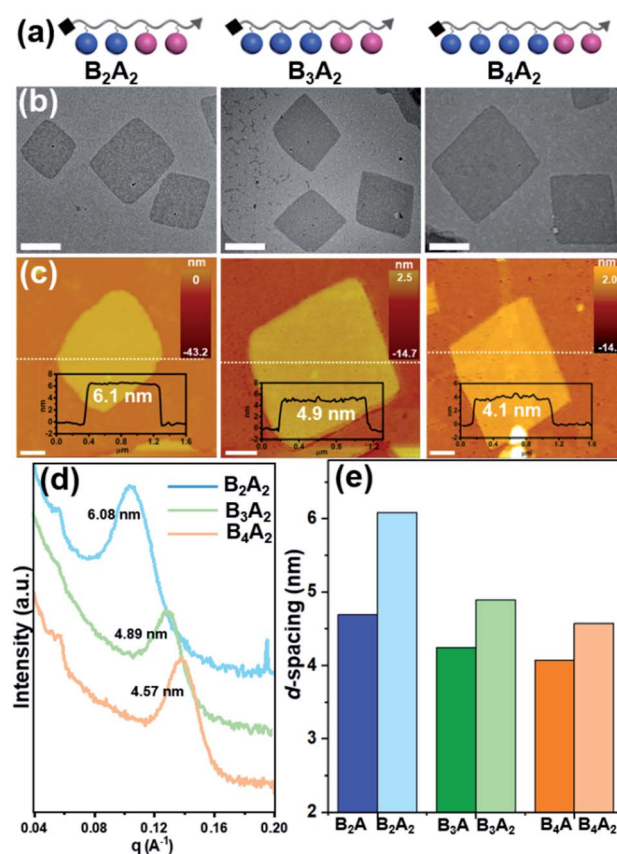
Fig. 5 Characterization of 2D nanosheets assembled from B n A 2 ( n = 2-4 ). (a) Cartoon illustrations of side-chain giant molecules B n A 2 ( n = 2-4 ). (b) TEM BF images of the 2D nanosheets (scale bar = 500 nm). (c) AFM images and height traces of the dashed lines shown as the insets (scale bar = 1 μm). (d) SAXS profiles collected from powder samples in transmission mode. Intensity is vertically offset for clarity. (e) Histograms of the 2D nanosheet thickness based on the SAXS data in (c) and Fig. 2d.
