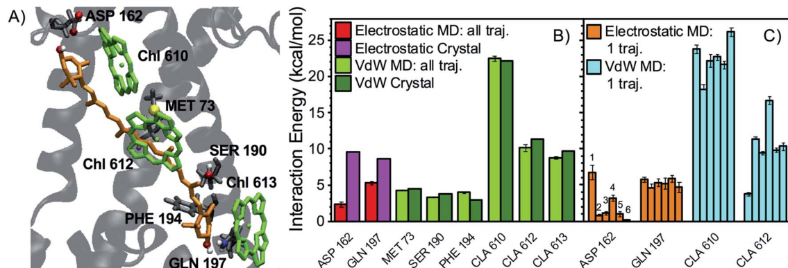
Fig. 3 Interaction partners of L1 lutein. (A) Binding pocket of L1 lutein in LHCII (coordinates from the optimized crystal structure) with the main interaction partners highlighted: Chls are in green, lutein in orange, while protein secondary structure and relevant residues are in gray, with the polar atoms of their side chains (as well as those of lutein) highlighted in red, blue, and white, for oxygen, nitrogen, and hydrogen atoms, respectively. (B) Average interaction energies of L1 lutein with selected residues. The red and light-green bars indicate the average electrostatic and vdW energies, respectively, over all cumulated MD snapshots, with their error bars indicating 96% confidence interval (2 times the standard error, with N = 323 ). The corresponding energies calculated on the crystal structure are shown in magenta and dark green. Only the interactions with an average >3.0 kcal mol ^{-1} over all MD snapshots are shown. Despite averaging below the latter threshold in the MD simulations, the electrostatic interaction energy between L1 lutein and ASP162 is also shown, as this pair gives rise to a strong HB according to the crystal structure and in a substantial fraction of MD snapshots. (C) average electrostatic and vdW interaction energies between L1 lutein and specific residues over each independent MD trajectory (the error bars indicate 96% confidence intervals, i.e. 2 times the standard error, with N = 60, 48, 53, 55, 55, 52 for trajectories 1–6, respectively).
