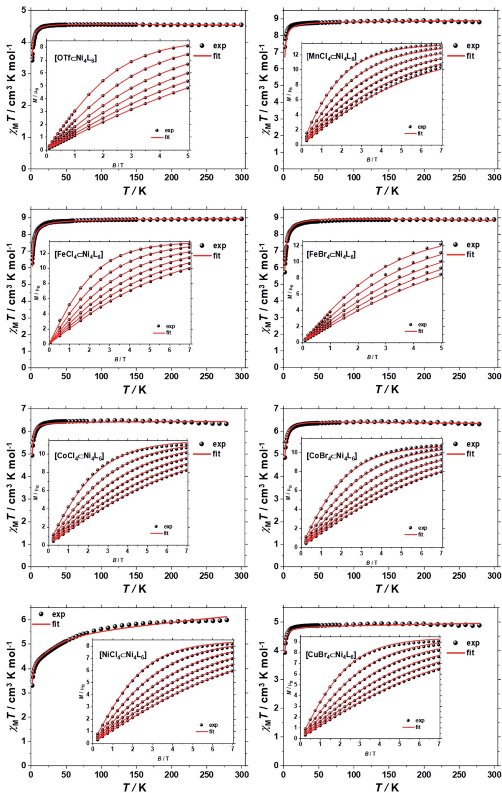
Fig. 3 \chi_M T versus T plots for [\text{OTf}]\text{Ni}_4\text{L}_6 (1) and [\text{M}^{\text{III}}\text{X}_4]\text{Ni}_4\text{L}_6 (2) (OTf) _6 , where \text{M}^{\text{III}}\text{X}_4^{2-} = \text{MnCl}_4^{2-} (2), \text{CoCl}_4^{2-} (5), \text{CoBr}_4^{2-} (6), \text{NiCl}_4^{2-} (7), \text{CuBr}_4^{2-} (8) or [\text{M}^{\text{III}}\text{X}_4]\text{Ni}_4\text{L}_6 (OTf) _7 , where \text{M}^{\text{III}}\text{X}_4^- = \text{FeCl}_4^- (3), \text{FeBr}_4^- (4) in the range T = 2\text{--}300 K and B = 0.1 T. The insets show the field dependence of the magnetisation measured in the T = 2\text{--}7 K and B = 0\text{--}7.0 T temperature and field ranges. The black spheres are the experimental data and the red lines the fit of the experimental data using spin-Hamiltonian (1), as explained in the text.
