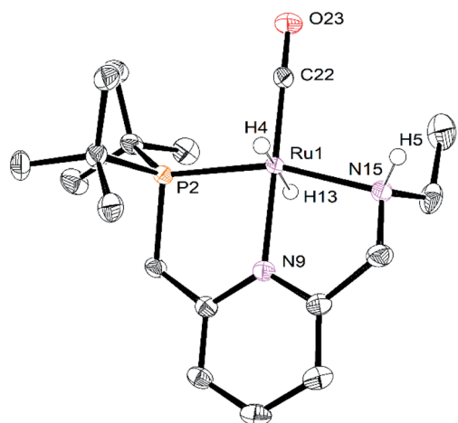
Fig. 6 ORTEP diagram of \text{RuPNN}^{\text{HEt}} , showing 50% probability ellipsoids. Hydrogen atoms other than \text{Ru-H} and \text{N-H} are omitted for clarity. Selected bond lengths (Angstroms) and angles (degrees): \text{Ru}(1)-\text{P}(2) , 2.2536(6); \text{Ru}(1)-\text{N}(15) , 2.1893(19); \text{Ru}(1)-\text{N}(9) , 2.0980(19); \text{Ru}(1)-\text{C}(22) , 1.830(2); \text{C}(22)-\text{O}(23) , 1.164(3); \text{P}(2)-\text{Ru}(1)-\text{N}(9) , 82.45(6); \text{N}(9)-\text{Ru}(1)-\text{N}(15) , 78.71(7).
