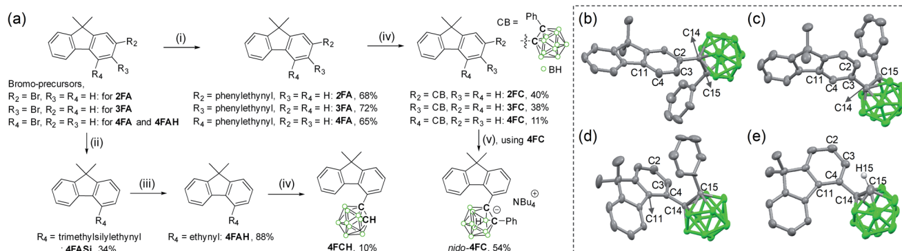
Scheme 1 Synthetic routes for the fluorene based o -carboranyl compounds. Reagents and conditions: (i) phenylacetylene, CuI, Pd(PPh 3 ) 2 Cl 2 , NEt 3 /toluene, 110 °C, 24 h. (ii) Ethynyltrimethylsilane, CuI, Pd(PPh 3 ) 2 Cl 2 , NEt 3 /toluene, 110 °C, 24 h. (iii) K 2 CO 3 , MeOH/DCM, 25 °C, 2 h. (iv) B 10 H 14 , Et 2 S, toluene, 120 °C, 24 h. (v) TBAF, THF, 60 °C, 24 h. The figures in the box show the molecular structures of (b) 2FC , (c) 3FC , (d) 4FC , and (e) 4FCH (50% thermal ellipsoids, solvent molecules in unit cell and H atoms were omitted for clarity).
