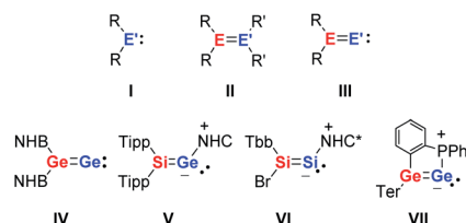
Fig. 1 Carbene analogues I , heteroalkenes II , heavy vinylidenes III ( E = Si, Ge ) and some examples of isolable sila- and germavinylidenes ( IV–VII ) (NHB = (HC(Dipp)N) 2 B, Tippi = 2,4,6-trisopropylphenyl, NHC = (MeC(iPr)N) 2 C, Tbb = 2,6-((Me 3 Si) 2 CH) 2 -4- tert -butylphenyl, NHC* = (H 2 C(Dipp)N) 2 C, Ter = 2,6-bis(2,4,6-trisopropylphenyl)phenyl, and Dipp = 2,6-diisopropylphenyl).
