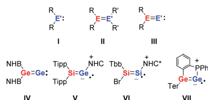
Fig. 1 Carbene analogues I , heteroalkenes II , heavy vinylidenes III ( E' = Si, Ge ) and some examples of isolable sila- and germavinylienes ( IV–VII ) (NHB = (HC(Dipp)N) 2 B, Tippi = 2,4,6-trisopropylphenyl, NHC = (MeC(iPr)N) 2 C, Tbb = 2,6-((Me 3 Si) 2 CH) 2 -4- tert -butylphenyl, NHC* = (H 2 C(Dipp)N) 2 C, Ter = 2,6-bis(2,4,6-trisopropylphenyl)phenyl, and Dipp = 2,6-diisopropylphenyl).
