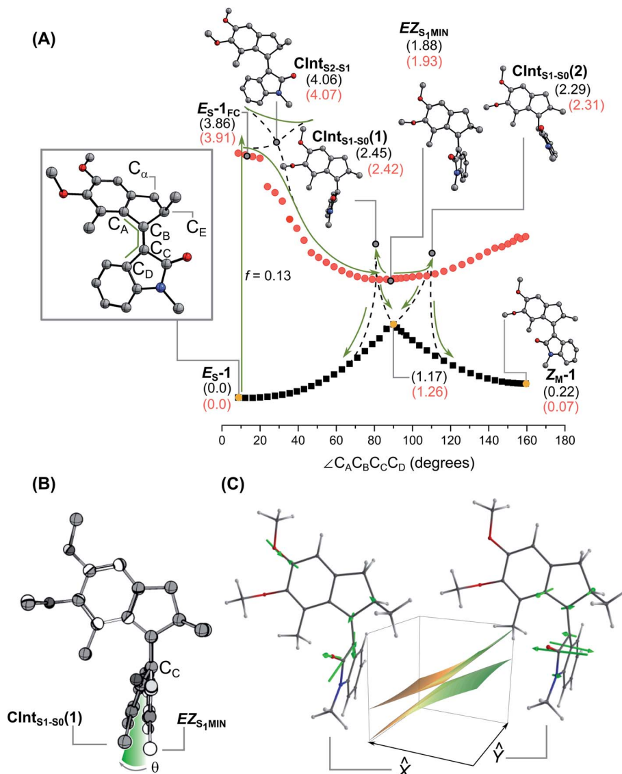
Fig. 6 Excited state isomerisation of E_5-1 . (A) Optimised S_0 and S_1 profiles along the rotation coordinate identified by the C_A C_B C_C C_D dihedral angle at the XMS-CASPT2/6-31G*///CASCF(12,12)/6-31G* level of theory. The relative energies in eV of the stationary points and CInts found along the relaxed scan are reported in parentheses (black: gas phase; red: single point using the PCM model for methanol). (B) Superposition of the geometry of EZ_{S1-MIN} (in white) and CInt_{S1-S0}(1) (in grey). The two structures mainly differ for their degree of pyramidalisation ( \angle \theta ) of C_C of the lower half. (C) Depiction of the branching plane of CInt_{S1-S2}(1) with the vectors \hat{x} and \hat{y} highlighted. Vector \hat{x} features the pyramidalisation distortion typical of the alkene branching plane, while vector \hat{y} describes the C_B=C_C bond twisting associated with the rotation. The sloped nature of the CInt can be appreciated by the tilting in the \hat{x} direction.
