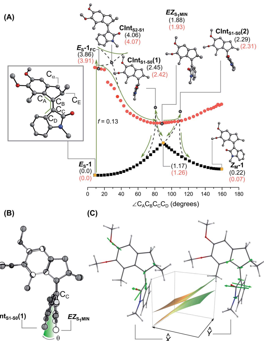
Fig. 6 Excited state isomerisation of E_5-1 . (A) Optimised S_0 and S_1 profiles along the rotation coordinate identified by the C_A C_B C_C C_D dihedral angle at the XMS-CASPT2/6-31G*///CASSCF(12,12)/6-31G* level of theory. The relative energies in eV of the stationary points and CInts found along the relaxed scan are reported in parentheses (black: gas phase; red: single point using the PCM model for methanol). (B) Superposition of the geometry of EZ_{S1-MIN} (in white) and Clnt_{S1-S0}(1) (in grey). The two structures mainly differ for their degree of pyramidalisation ( \angle \theta ) of C_C of the lower half. (C) Depiction of the branching plane of Clnt_{S1-S2}(1) with the vectors \hat{x} and \hat{y} highlighted. Vector \hat{x} features the pyramidalisation distortion typical of the alkene branching plane, while vector \hat{y} describes the C_B=C_C bond twisting associated with the rotation. The sloped nature of the CInt can be appreciated by the tilting in the \hat{x} direction.
