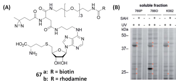
Fig. 18 Gel-based analysis of MTs was performed using AfBPs. (A) Structures of reported AfBPs for MTs. (B) Gel-based profiling with 67b in human renal cancer cell (769P and 786O) and human leukemia cell (K562) lysates. 67 successfully labeled MTs in a variety of cancer cells. The addition of SAH (natural substrate) or the lack of UV irradiation resulted in the loss of MT labeling. Reproduced from ref. 167 with permission from American Chemical Society, copyright 2019.
