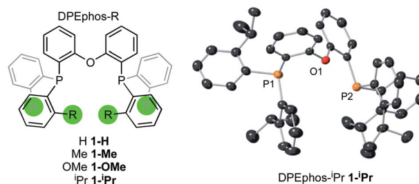
Fig. 3 DPEphos-R ligands used in this study. Crystallographically determined structure of 1- i Pr . Ellipsoids shown at the 50% probability level. Hydrogen atoms omitted for clarity. See ESI † for full details.
