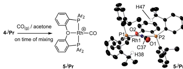
Scheme 4 Reaction of 4- i Pr with CO, and solid-state structure of 5- i Pr highlighting the position of anagostic contacts. [BAR F 4 ] - anions not shown. Displacement ellipsoids are shown at the 50% probability level. Rh1-P1, 2.3145(7); Rh1-P2, 2.3027(8); Rh1-C37, 1.819(4); Rh1-O2, 2.128(3); Rh-H38, 2.821; Rh-H47, 2.627; P1-Rh1-P2, 162.41(4); O2-Rh1-C1, 177.0(1).
