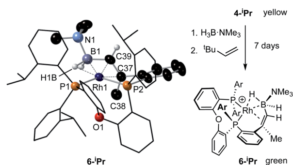
Scheme 6 Synthesis and solid-state structure of 6- 1 Pr. Displacement ellipsoids are shown at the 30% probability level. Selected bond distances and angles: Rh1-P1, 2.3361(9); Rh1-P2, 2.2696(11); Rh1-B1, 2.391(6); Rh1-C37, 2.266(3); Rh1-C39, 2.152(3); Rh1-H1B, 1.99(5); B1-C39, 1.557(6); C37-C38, 1.511(6); C37-C39, 1.392(6); P1-Rh1-P2, 100.59(4); B1-C39-C37, 123.2(3); Rh1-H1B-B1, 87.8(18).
