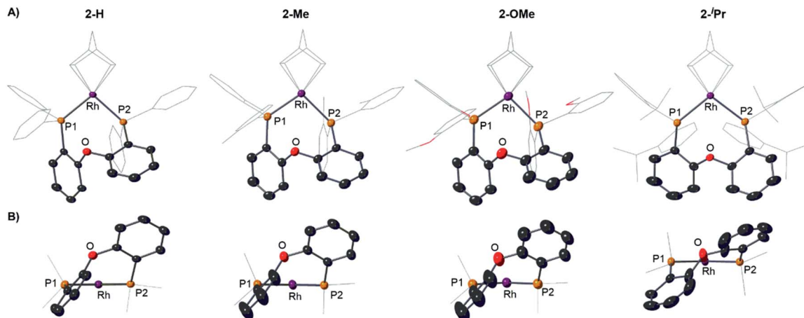
Fig. 4 (A) Solid-state structures of the cations in 2-H, 2-Me, 2-OMe and 2- 1 Pr as determined by single-crystal X-ray diffraction. Displacement ellipsoids are shown at the 50% probability level. Hydrogen atoms and [BAR 4 ] − anions not shown. Selected DPEphos-R and NBD groups shown as wireframe. (B) End-on view highlighting the relative orientation of the DPEphos backbones. Bond lengths and angles are given in the ESI (Table S2). †
