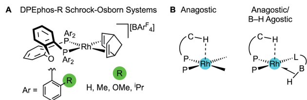
Fig. 2 (A) [Rh(DPEphos-R)(NBD)][BAR F 4 ] systems, and (B) schematic examples of the C–H anagostic interactions and 3c-2e B–H agostic bonds, reported in this contribution.
