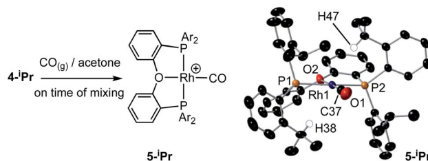
Scheme 4 Reaction of 4- i Pr with CO, and solid-state structure of 5- i Pr highlighting the position of anagostic contacts. [BAR F 4 ] - anions not shown. Displacement ellipsoids are shown at the 50% probability level. Rh1–P1, 2.3145(7); Rh1–P2, 2.3027(8); Rh1–C37, 1.819(4); Rh1–O2, 2.128(3); Rh–H38, 2.821; Rh–H47, 2.627; P1–Rh1–P2, 162.41(4); O2–Rh1–C1, 177.0(1).
