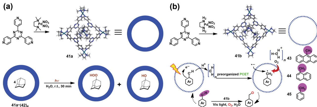
Fig. 14 (a) Schematic representation of the radical-mediated photooxidation of adamantane 42 within a coordination cage 41a containing a redox-active triazine core. Reproduced from ref. 50. (b) Schematic representation of the photoactivation of C–H bonds inside water-soluble nanocage 41b and its mechanism. Reproduced from ref. 51.
