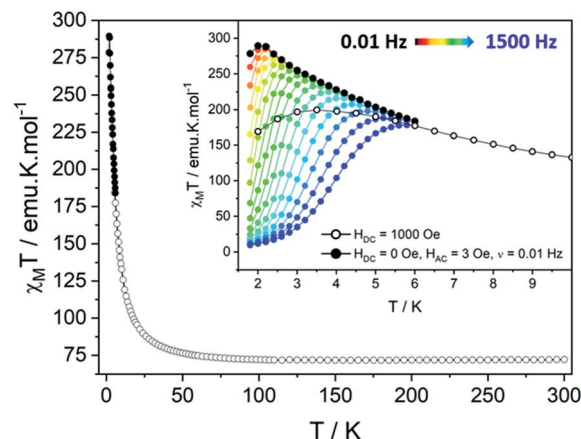
Fig. 6 (Top) Temperature dependence of \chi_M T for the hexanuclears measured with H_{\text{dc}} = 1000 \text{ Oe} (black circles) and reconstructed from ac measurements with H_{\text{dc}} = 0 \text{ Oe} , H_{\text{ac}} = 3 \text{ Oe} , \nu = 0.01 \text{ Hz} (black dots). In inset, a zoom in the low temperature region with the ac data for frequencies from \nu = 0.01 \text{ Hz} (black) to 1500 \text{ Hz} (blue).
