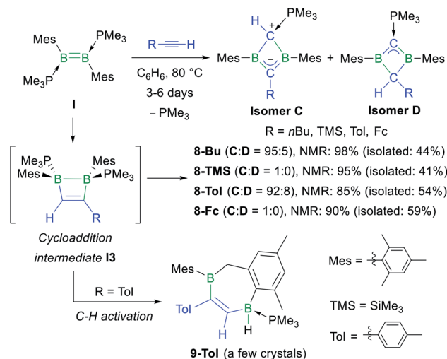
Scheme 6 Reaction of phosphine-stabilised diborene I with terminal acetylenes, postulated intermediate I3 in square brackets, and C–H activation product 9-Tol deriving from I3 . Relative stereochemistry shown only.
