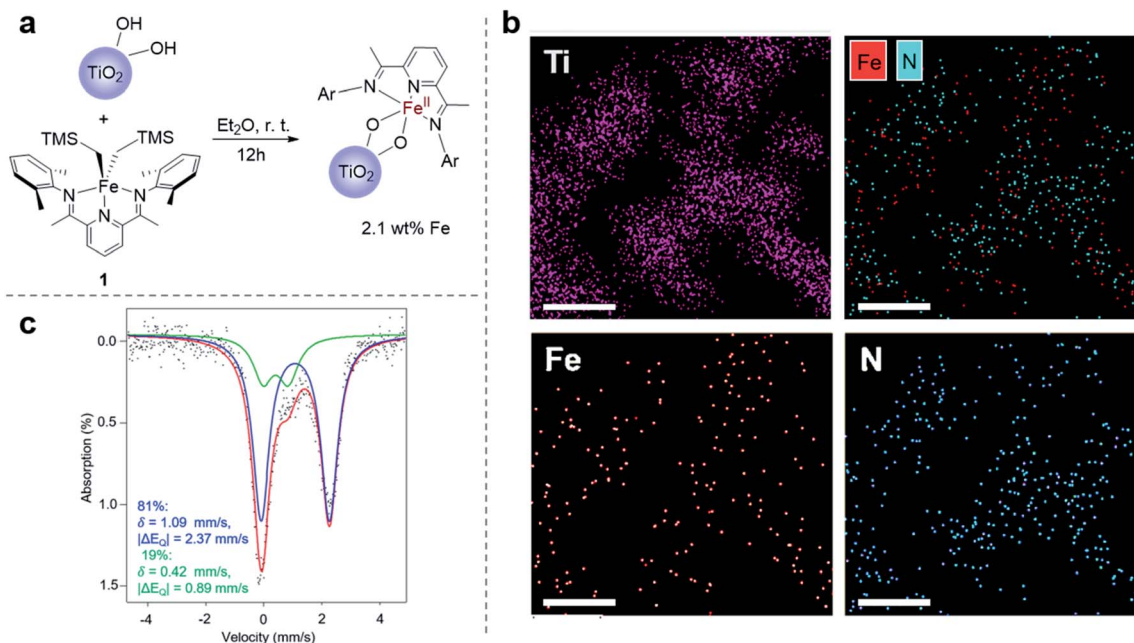
Fig. 1 (a) Reaction scheme for anchoring the molecular iron complex onto P25 \text{TiO}_2 nanoparticle (Ar = 2,6-dimethylphenyl); (b) STEM elemental mapping of the \text{Fe(II)}-\text{TiO}_2 powder (scale bar: 50 nm); (c) Mössbauer spectroscopy of \text{Fe(II)}-\text{TiO}_2 powder.
