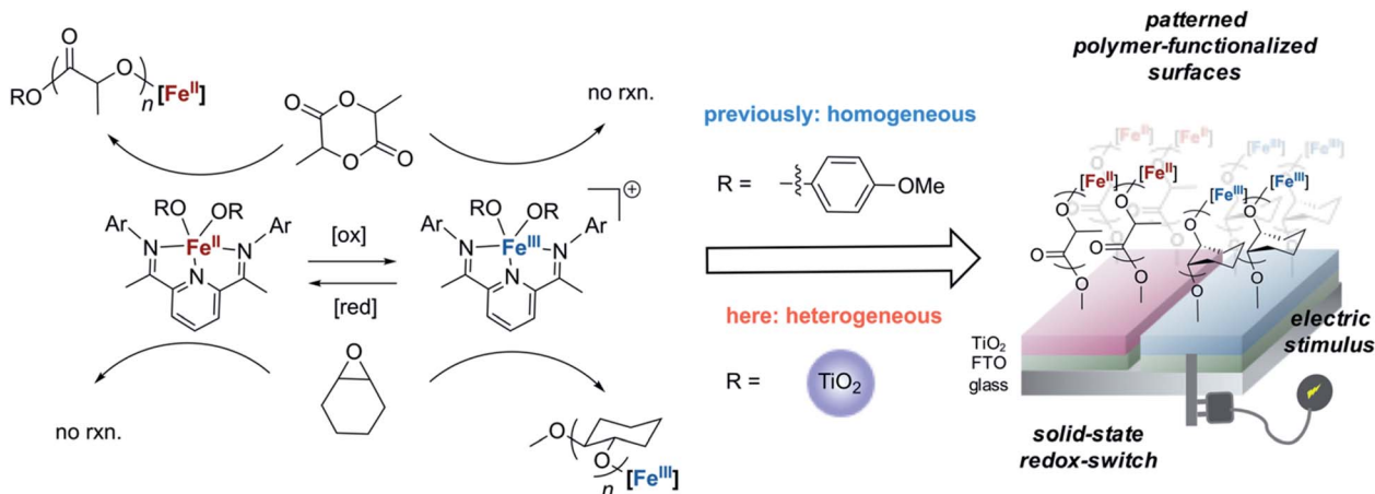
Scheme 1 Iron-based catalysts reported for the redox-switchable polymerization of lactide and epoxides 38,40 are extended to the solid state by appending iron-based catalysts to titanium dioxide nanoparticles. Application of an electric stimulus to a conducting substrate containing electrically isolated zones coated with these particles enables patterning of surfaces with two different polymer brushes.
