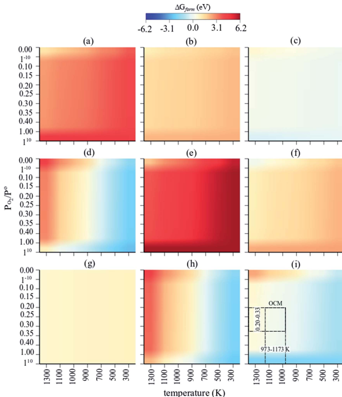
Fig. 2 Individual heat maps of computed Gibbs free energy of formation for (\text{Mn}_b\text{O}_b-\text{Na}_2\text{WO}_4)/\text{SiO}_2 as a function of T (300–1300 K) and P_{\text{O}_2}/P = 0-1 (ref. 10) for (a) Mn, (b) MnO, (c) \text{MnO}_2 , (d) \text{MnO}_3 , (e) \text{Mn}_2\text{O} , (f) \text{Mn}_2\text{O}_2 , (g) \text{Mn}_2\text{O}_3 , (h) \text{Mn}_2\text{O}_4 , (i) \text{Mn}_2\text{O}_5 . The dashed rectangle in (i) signifies the OCM relevant conditions.
