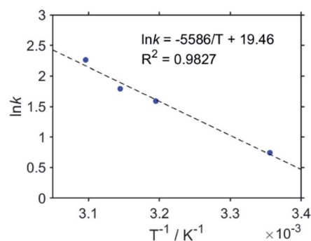
Fig. 11 Arrhenius plot from which k_c is derived.
