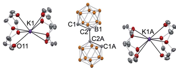
Fig. 5 Displacement ellipsoid plot (50% probability) of [\text{K}(12\text{-crown-4})_2]_2(\text{C}_2\text{B}_{10}\text{H}_{10})_2 \cdot 4(\text{THF}) (6). Note the lack of \text{C} \cdots \text{K} contact and the complete ion separation. Only a half of the asymmetric unit is shown. Hydrogen atoms on boron atoms of the cluster and carbon atoms of the crown ether ligand have been omitted for clarity. Crystallization solvent molecules (THF) are not shown. Selected interatomic distances (Å): \text{K1} \cdots \text{C1} = 6.283(1) , \text{C1} - \text{C2} = 1.712(1) , \text{C1} - \text{B1} = 1.724(2) , \text{C2} - \text{B1} = 1.698(2) , \text{C2} - \text{C2A} = 1.532(2) Å.
