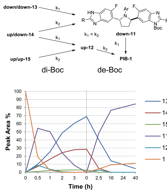
Scheme 3 De-Boc of di-Boc mixture to give 11 selectively. De-Boc conditions: n -BuNH 2 (1.5 equiv.), MTBE (8 mL g -1 ), 23 °C.
