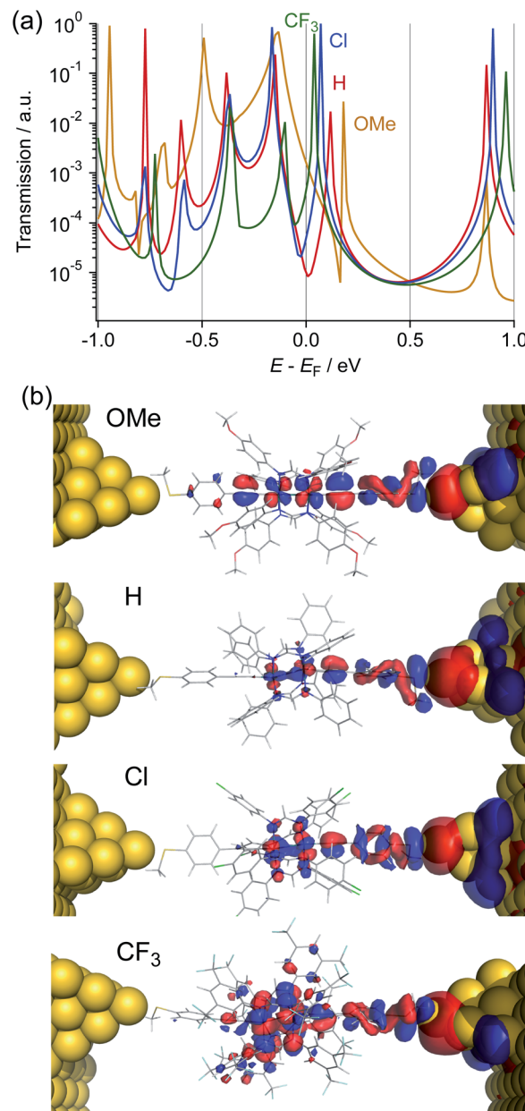
Fig. 8 (a) Transmission spectra and (b) the dominant transmission eigen channel at the Fermi level of Au-1 R - Au ( R = \text{OMe}, \text{H}, \text{Cl}, \text{and CF}_3 ).
