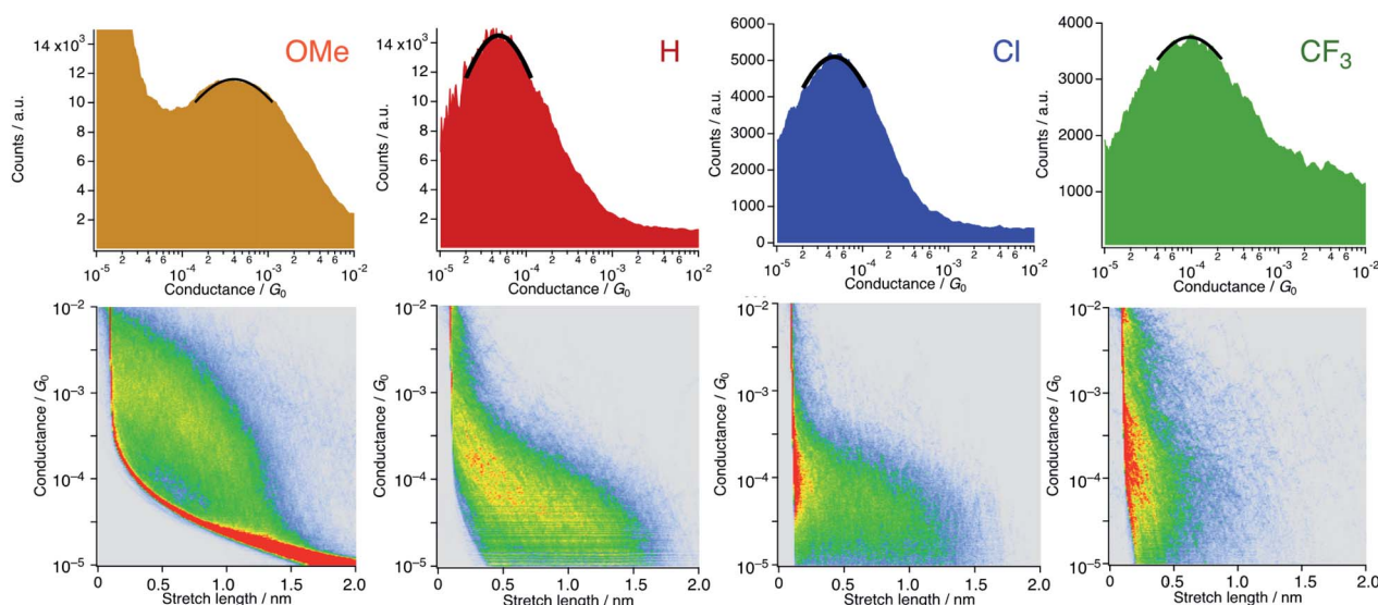
Fig. 4 1D and 2D histograms of \mathbf{1}^R ( X = \text{OMe} , \text{H} , \text{Cl} , and \text{CF}_3 ) constructed from 2000 successive traces. [ \mathbf{1}^R ] = 0.25 mM in tetraglyme. No data selection was performed.
