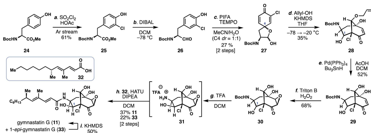
Scheme 1 Total synthesis of gymnastatin G.
