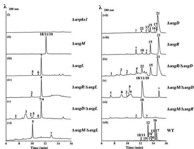
Fig. 2 HPLC-MS profiles (UV 280 nm) of the gene-deletion mutants. For traces (ii) and (x), 18, 11, and 10 were resolved by using a different column (Fig. S15 and S17†). For trace (v), 7 and 4 were resolved likewise (Fig. S16†). * – unrelated peaks. WT: wild type.
