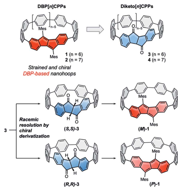
Fig. 1 DBP[ n ]CPPs 1 and 2 as strained and chiral dibenzo[ a,e ]pentalene-based hoops, which can be accessed from diketo[ n ]CPPs 3 and 4. Their racemic resolution by chiral derivatization of the carbonyl groups provides access to enantiopure nano hoops.
