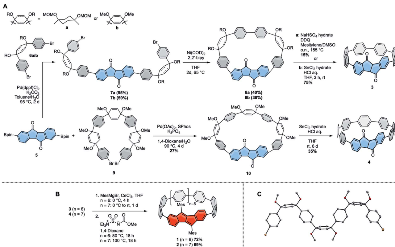
Scheme 1 Synthesis of diketo[ n ]CPPs 3 and 4 (A) and DBP[ n ]CPPs 1 and 2 (B) ( 5 was used as a racemic mixture, hence all derived compounds are racemic. For simplicity, a single enantiomer is shown for 1–4); (C) molecular structure of 9 in the solid state (displacement ellipsoids are shown at the 50% probability level; hydrogen atoms are omitted for clarity).
