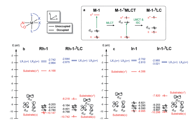
Fig. 7 (a) Electronic excitations and (b) frontier molecular orbitals of \text{M-1} computed at the B3LYP-D3/cc-pVTZ(-f)/LACV3P** level of theory.
