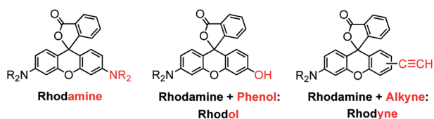
Chart 1 The molecular structures of rhodamine, Rhodol, and a new rhodamine-like dye with an alkyne substituent on the xanthenone unit (named Rhodyne).
