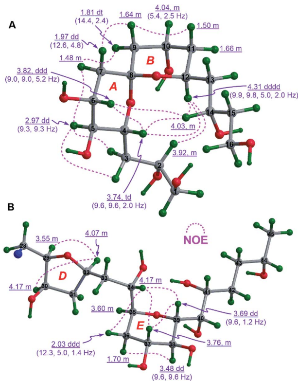
Fig. 3 (A) The relative configuration of the 6,6-spiroketal moiety in 1a and (B) those of rings D and E in 1b assigned by diagnostic NOE interactions and ^3J_{\text{H,H}} values (the C17 to C27 moiety in 1b is omitted for clarity).
