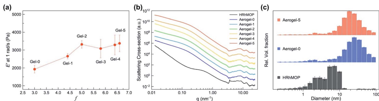
Fig. 3 (a) Evolution of storage Young's modulus ( E' at 1 rad s -1 ) of Gel- n as a function of f during repeated aging process. (b) SXAS/WAXS curves of HRhMOP and Aerogel- n (the data was stacked for clarity, all data on an absolute intensity scale can be found in ESI†). (c) Form-free size distributions of HRhMOP, Aerogel-0 and Aerogel-5 extracted from SAXS fits from Monte Carlo method.
