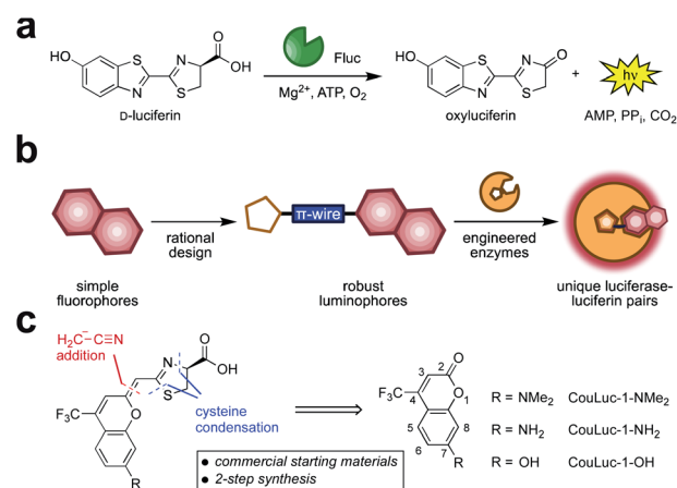
Fig. 1 Red-emitting orthogonal bioluminescent probes designed from fluorophores. (a) D-Luciferin is oxidized by firefly luciferase (Fluc) to produce oxyluciferin and a photon of light. (b) Coumarin fluorophores were used as templates for red-shifted luciferins. (c) Retrosynthetic analysis of the CouLuc-1 analogs.
