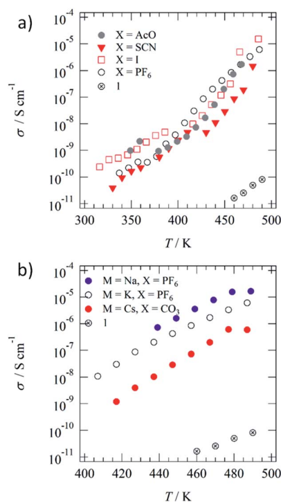
Fig. 2 Temperature-dependent ionic conductivity of M^+ \cdot (1) \cdot X^- . (a) Anion ( X^- )-dependent \sigma_{ion}-T plots of K^+ \cdot (1) \cdot X^- ( X^- = AcO^-, SCN^-, I^- , and PF_6^- ) and K^+ -free 1 . (b) Cation ( M^+ )-dependent \sigma_{ion}-T plots of Na^+ \cdot (1) \cdot PF_6^- , K^+ \cdot (1) \cdot PF_6^- , Cs^+ \cdot (1) \cdot (CO_3^{2-})_{0.5} , and M^+ -free 1 .
