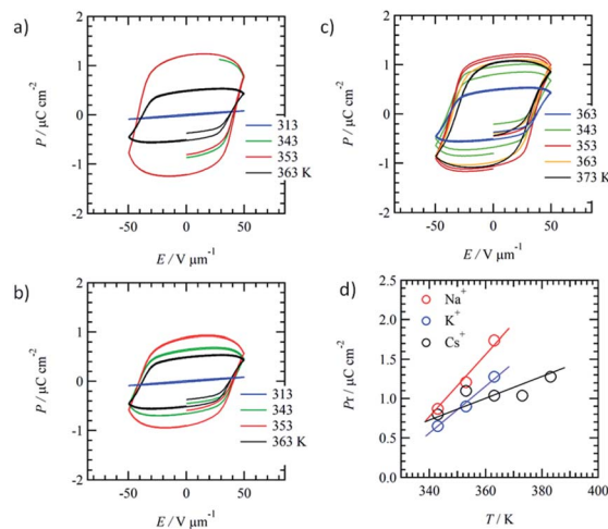
Fig. 5 Temperature-dependent P-E hysteresis curves of ion-doped mixed crystals of (a) (\mathbf{3BC})_{0.9}[(\text{Na}^+)_{0.5}(\mathbf{1}) \cdot (\text{PF}_6^-)_{0.5}]_{0.1} , (b) (\mathbf{3BC})_{0.9}[(\text{K}^+)_{0.5}(\mathbf{1}) \cdot (\text{PF}_6^-)_{0.5}]_{0.1} , and (c) (\mathbf{3BC})_{0.9}[(\text{Cs}^+)_{0.5}(\mathbf{1}) \cdot (\text{CO}_3^{2-})_{0.25}]_{0.1} . (d) Temperature-dependent P_r values of \text{Na}^+ , \text{K}^+ , and \text{Cs}^+ -doped (\mathbf{3BC})_{0.9}(\mathbf{1})_{0.1} .
