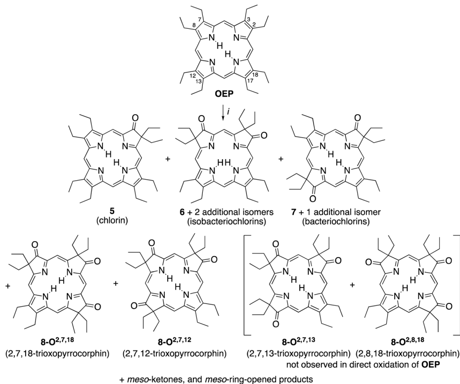
Scheme 2 Oxidation of octaethylporphyrin OEP to the corresponding \beta -oxo derivatives. 10a,15 Reaction conditions: (i) (1) \text{H}_2\text{O}_2 (3%)/ \text{H}_2\text{SO}_4 (96%), ~15 min, 0 °C. (2) \text{NaOAc} , \text{H}_2\text{O} . (3) Chromatography. The atom numbering in octaethylporphyrin OEP shows the numbering system used, the basis for the \beta -ketone names.
