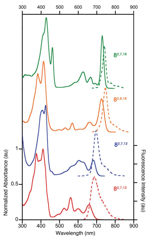
Fig. 3 Normalized UV-vis absorption (solid trace) and fluorescence emission (broken trace) spectra of the trioxopyrrocorphins indicated (all in \text{CH}_2\text{Cl}_2 ); \lambda_{\text{excitation}} = \lambda_{\text{Soret-max}} . For their extinction coefficients, see ESI†
