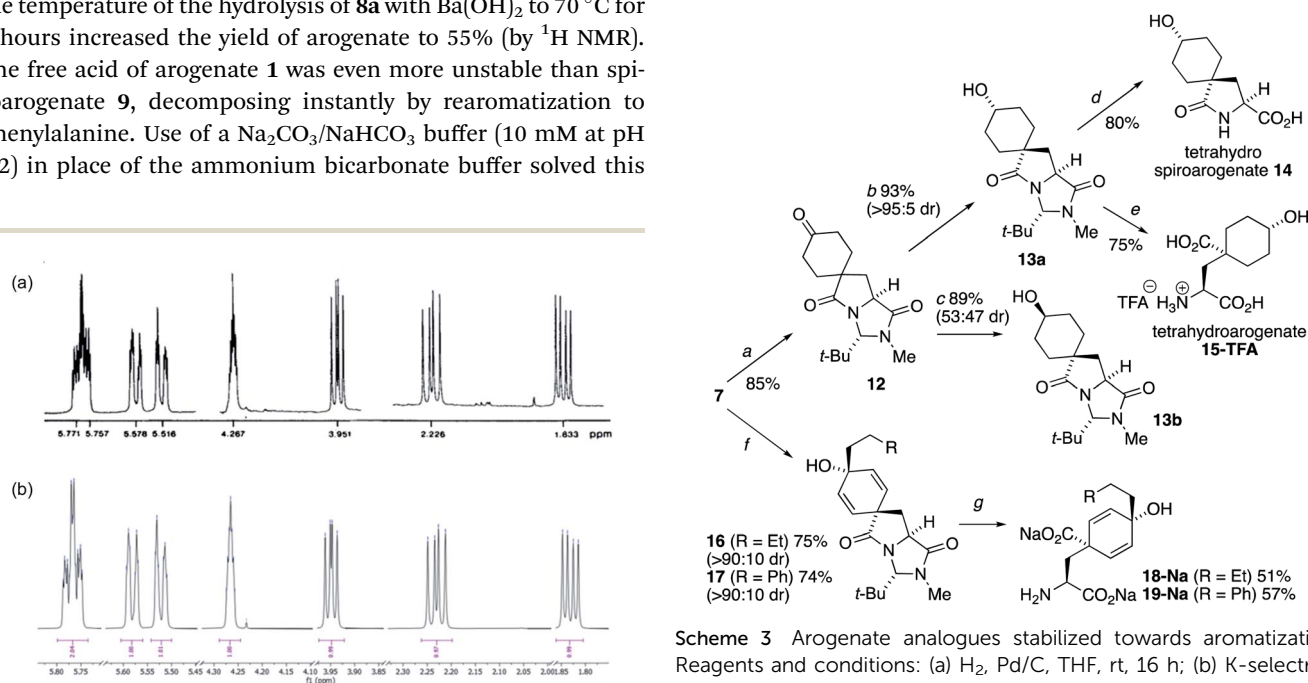
Fig. 2 1 H NMR spectrum of spiroarogenate 9 (a) isolated from Neurospora crassa (400 MHz in D 2 O); 19 (b) synthesized by the method of Scheme 2 (400 MHz in D 2 O).
