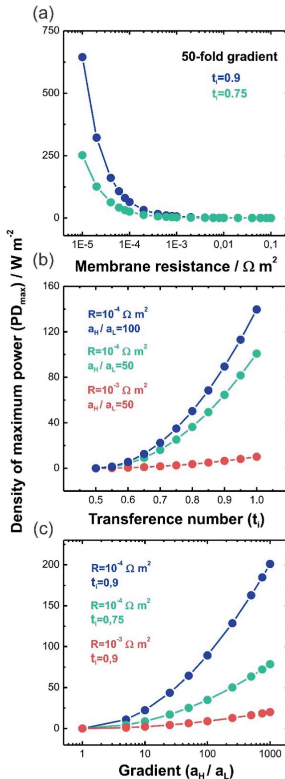
Fig. 4 Density of maximum power ( PD_{\text{max}} ) predicted by eqn (27) as a function of (a) membrane resistance ( R ), (b) transference number and (c) gradient concentration ( a_H/a_L ) ( T = 298 K).
