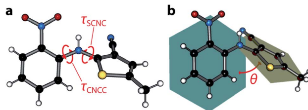
Fig. 1 (a) Molecular structure of ROY. Carbon atoms are shown in black, nitrogen in blue, oxygen in red, sulfur in yellow, and hydrogen in white. The two rotatable bonds \tau_{\text{SCNC}} and \tau_{\text{CNCC}} that can influence intramolecular conjugation are indicated. (b) An alternate measure of the extent of ring coplanarity; the angle \theta between mean planes calculated through the phenyl and thiophene groups.
