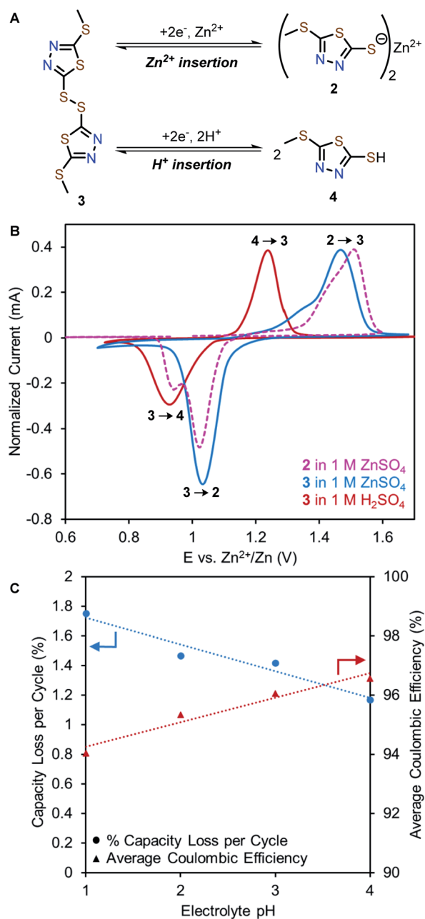
Fig. 5 (A) Possible \text{Zn}^{2+} and \text{H}^+ insertion products derived from reduction of 3. (B) Solid state CV of 2 measured in a two-electrode cell with 1 M \text{ZnSO}_4 electrolyte (pink dotted line) and 3 measured in a three-electrode cell with 1 M \text{ZnSO}_4 (blue solid line) or 1 M \text{H}_2\text{SO}_4 electrolytes (red solid line). The position of the 1 M \text{H}_2\text{SO}_4 curve is adjusted to represent a dilute \text{H}_2\text{SO}_4 solution (pH = 4), calculated based on the Nernst equation. Current is normalized to oxidation peak for consistency. (C) pH-dependent capacity loss and coulombic efficiency of Zn-2 cells.
