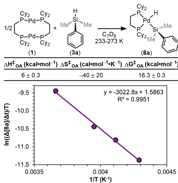
Fig. 13 Eyring plot constructed from variable temperature kinetics data in C 7 D 8 (13.33 mM). Product concentration was determined by 31 P ( 1 H) NMR integration against an internal standard; 1.00 equiv. of 1 and 2.05 equiv. of 3a was used. \Delta G_{\text{OA}}^\ddagger determined at 233 K.
