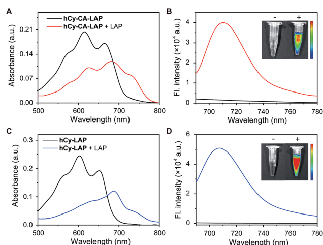
Fig. 1 In vitro response of hCy-CA-LAP and hCy-LAP toward LAP. Absorption spectra and fluorescence spectra of hCy-CA-LAP (A and B) and hCy-LAP (C and D) (10 \mu\text{M} ) in the absence and presence of LAP (0.2 U \text{mL}^{-1} , \lambda_{\text{ex}} = 680 nm). (Insets B and D) NIR fluorescence images of the two probes before and after reacting with LAP, \lambda_{\text{ex}} = 640 nm and \lambda_{\text{em}} = 740 nm. All spectra were recorded in PBS buffer (10 mM, pH = 7.4, containing 1% DMSO) at 37 ^{\circ}\text{C} .
