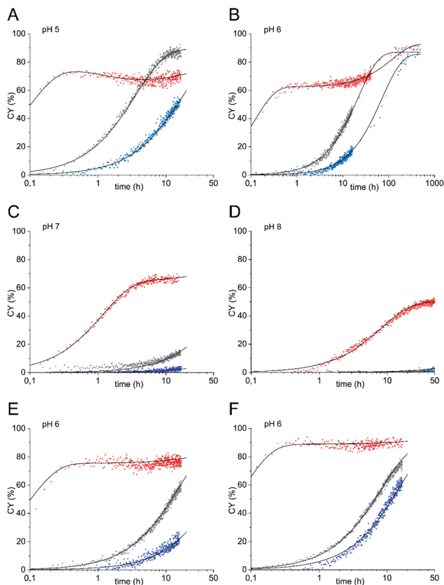
Fig. 3 Oxyamine ligation reaction of glycosyl amine 10 (red) and GlcNAc with 100 mM aniline (grey) or without aniline (blue) (5 mM sugar) with 10 equiv. of ethoxyamine at (A) pH 5, (B) pH 6, (C) pH 7, (D) pH 8, and at pH 6 with 20 equiv. (E) and 50 equiv. of ethoxyamine (F).
