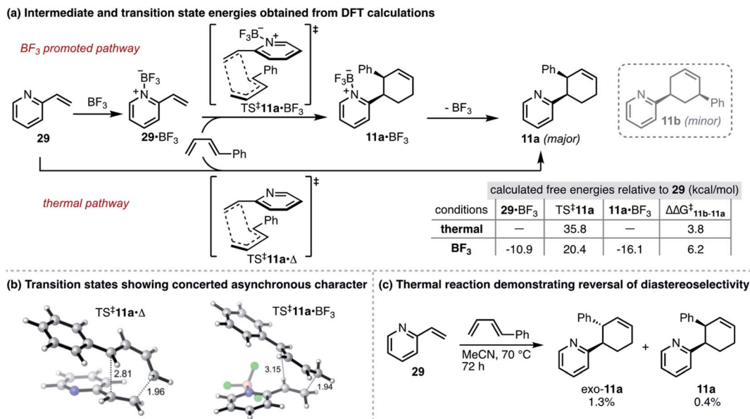
Scheme 1 (a) Thermal vs. \text{BF}_3 -promoted pathways: summary of DFT calculations for formation of 11a . Transition state energies provided reflect concerted, endo cycloadditions consistent with observed products. Calculations carried out using Gaussian 16, using the B3LYP functional with the 6-311+G(d) basis set with a solvent model using the dielectric constant for acetonitrile. See ESI† for details. (b) Transition states for endo cycloadditions of 2-vinylpyridine and 1-phenylbutadiene, showing half-formed \sigma -bonds as dashed lines, with bond lengths in Å. Hydrogens in white, carbons in grey, nitrogen in blue, boron in pink and fluorine in green. (c) Results for thermal cycloaddition between 29 and 1-phenylbutadiene at 70 °C.
