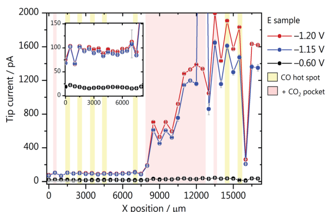
Fig. 5 SECM array scans through the catalyst gradient of GDE-B at a \text{CO}_2 back-pressure of 4.2 mbar. The applied GDE potentials were -1.2 V (red), -1.15 V (blue) and -0.6 V (black), reported versus Ag/AgCl/3 M KCl and measurements were performed in 1 M \text{KHCO}_3 . CO hot spots and \text{CO}_2 pockets are marked with a yellow and red shade, respectively.
