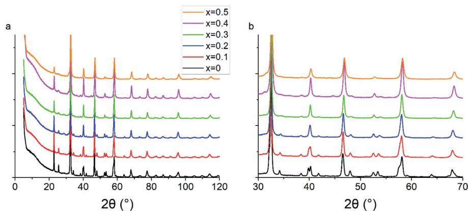
Fig. 1 (a) Powder XRD patterns for the as-synthesised Pr 1- x Sr x FeO 3- \delta perovskite oxides. (b) As the concentration of strontium ( x ) increases, there is a phase transformation towards a high symmetry pseudo-cubic structure, as seen by the reduction in the number of visible Bragg reflections around for example 2\theta = 40.2, 47.9 and 53.4^\circ .
