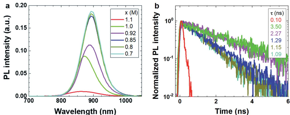
Fig. 4 PL measurements of \text{PEA}_{0.08}\text{FA}_x\text{SnI}_3 films. (a) Steady state and (b) time-resolved PL. The color scheme is the same in the two figures, lifetimes are reported in the legend of (b).
