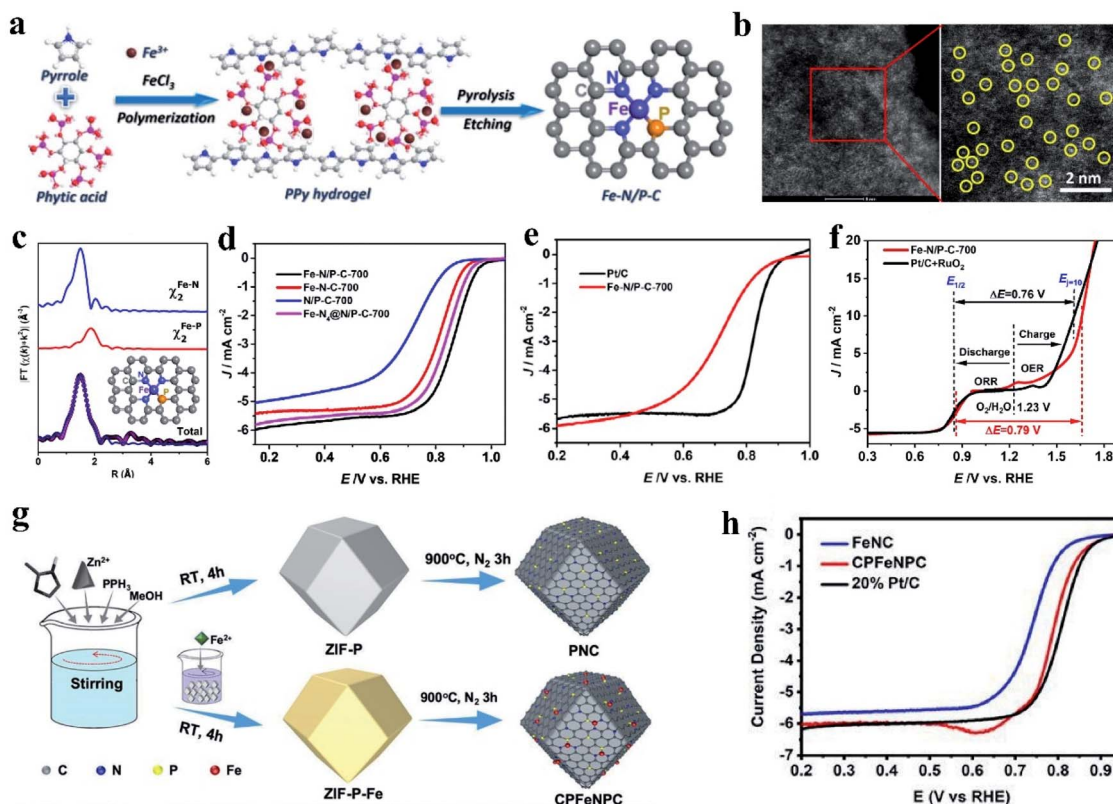
Fig. 2 (a) Schematic of the synthesis of the Fe–N/P–C catalyst. (b) Aberration-corrected HAADF-STEM image and enlarged image of Fe–N/P–C-700, partial single Fe atoms are circled in yellow. (c) EXAFS analysis of Fe–N/P–C-700 at R space. (d) ORR polarization curves of Fe–N/P–C-700, Fe–N–C-700, N/P–C-700, and Fe–N 4 @N/P–C-700 catalysts at a rotating speed of 1600 rpm in 0.1 M KOH solution. (e) LSV curves of Fe–N/P–C-700 and Pt/C. (f) Overall polarization plots (1600 rpm) in the ORR and OER potential window for Fe–N/P–C-700 and commercial Pt/C + RuO 2 catalysts, and the inset depicts the overall electrocatalytic oxygen performance ( \Delta E = E_j = 10 - E_{1/2} ). Reproduced with permission. 131 Copyright 2020, the American Chemical Society. (g) Preparation of PNC and CPFenPC. (h) ORR activities of the PNC and CPFenPC catalysts in 0.1 M KOH electrolyte. Reproduced with permission. 133 Copyright 2020, The Royal Society of Chemistry.
