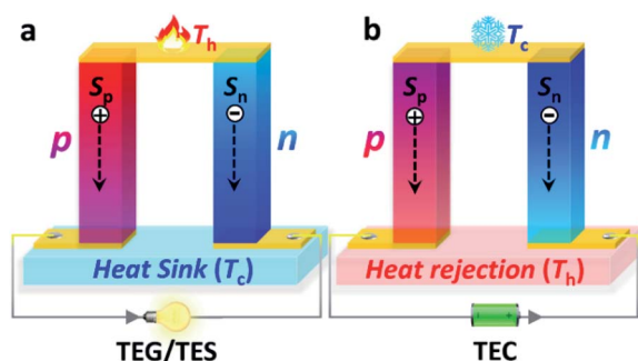
Fig. 1 Schematic illustration of the physical processes of TE unicouples used for (a) TEGs/TESs and (b) TECs.
