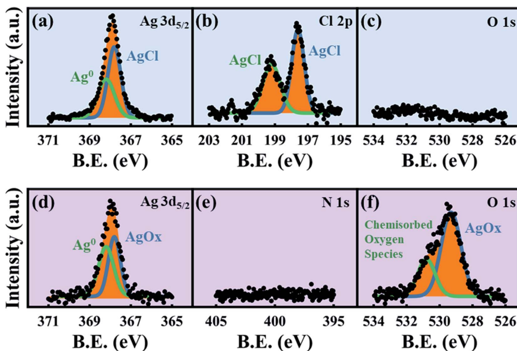
Fig. 6 XPS spectra. Top row is for the \text{HClO}_4 -dealloyed ex situ sample: (a) Ag 3d_{5/2} , (b) Cl 2p and (c) O 1s, demonstrating AgCl growth even in larger electrolyte volumes. Bottom row is for the \text{HNO}_3 -dealloyed ex situ sample: (d) Ag 3d_{5/2} , (e) N 1s and (f) O 1s, demonstrating that there is no nitrogen-containing surface coating.
