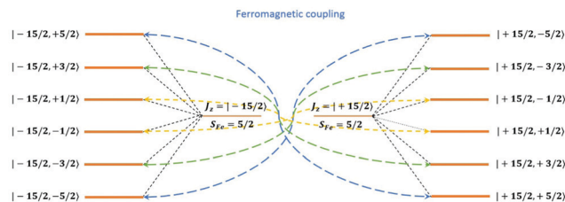
Fig. 14 Energy splitting of the lowest manifold arising from the exchange coupling between a strong anisotropic lanthanide ion (e.g., Dy^{III} ) and a transition metal ion (e.g., Fe^{III} ) in weak ZFS. Here orange lines are energy levels, colored lines with arrows indicates the most preferred relaxation channel for population at corresponding energy level. Lines with the same color are expected to have the same transition rate. Dominant path is the competition between different colored lines. Effective blocking barrier can thus range from the height of the fourth to the sixth energy levels depending on the specific system and temperature.
