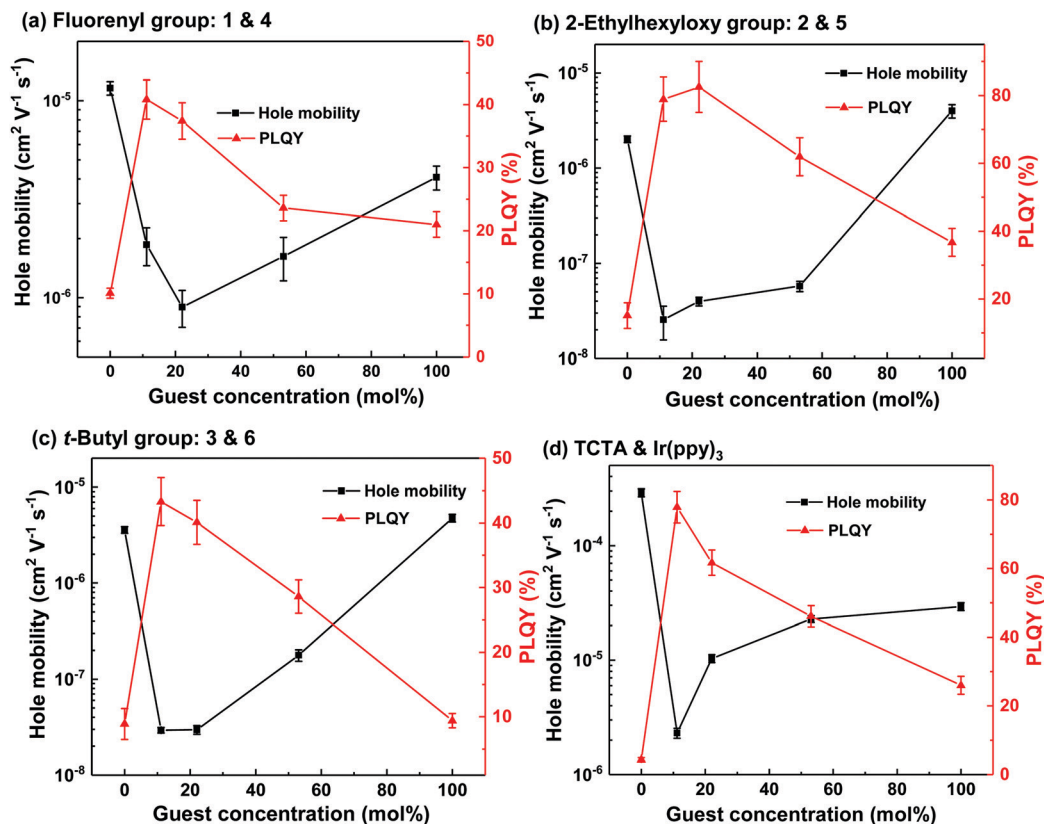
Fig. 4 Mobility and PLQY values of neat and blend films of 1 and 4 (a), 2 and 5 (b), 3 and 6 (c) and TCTA and \text{Ir}(\text{ppy})_3 (d) at different concentrations. Fig. (d) was reproduced with permission. 26,27
